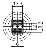
Terminal Arrangement
